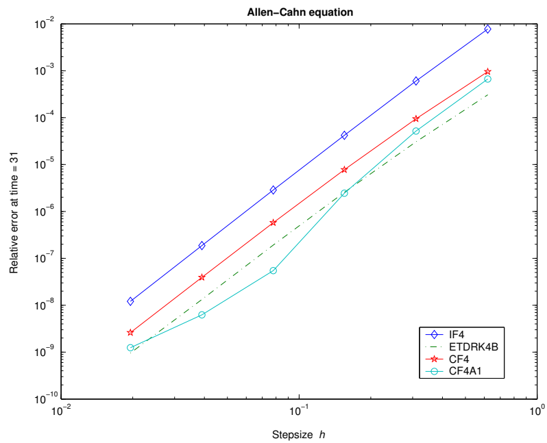
Figure 2: Step size versus relative error for fourth order methods for the Allen-Cahn equation
