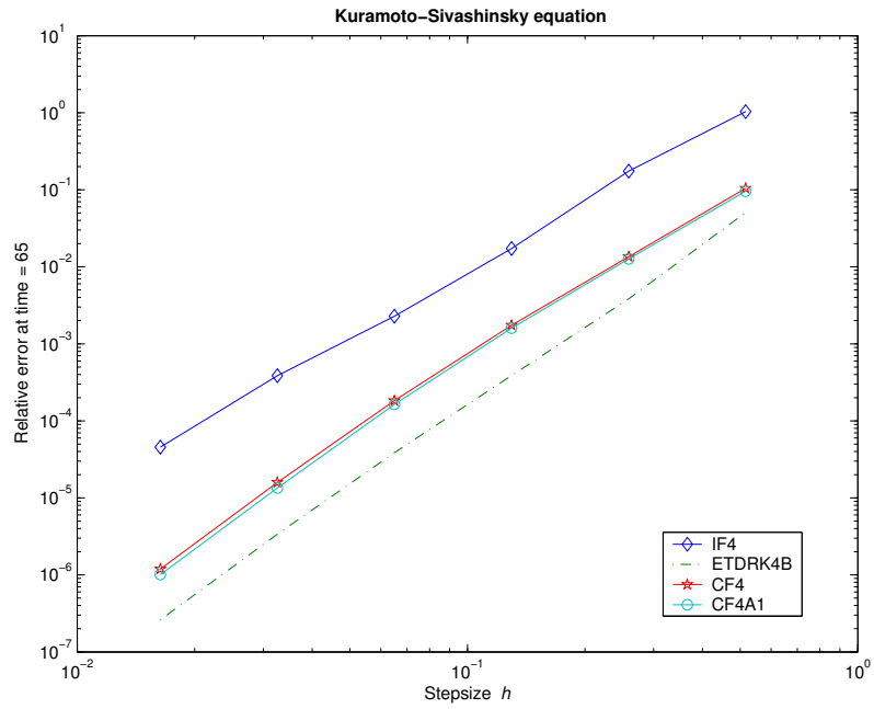
Figure 1: Step size versus relative error for fourth order methods for the Kuramoto-Sivashinsky equation
